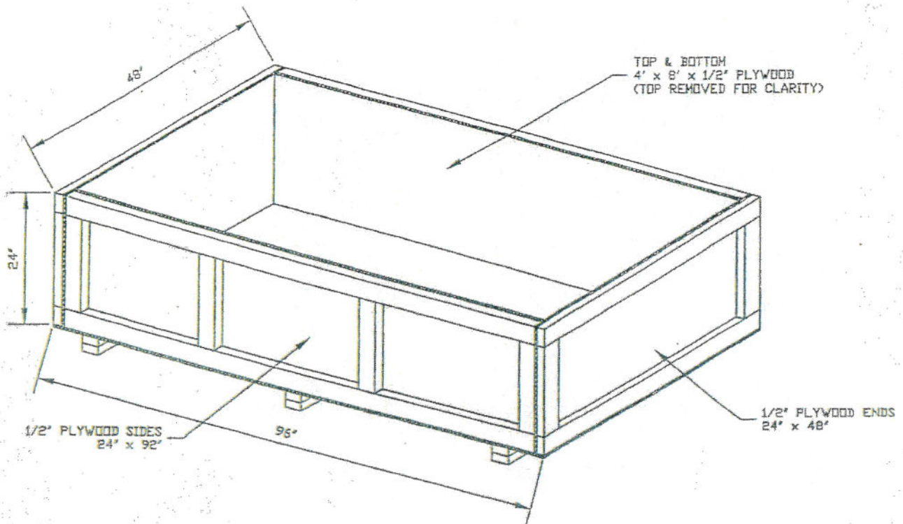
SHIPPING CRATE
